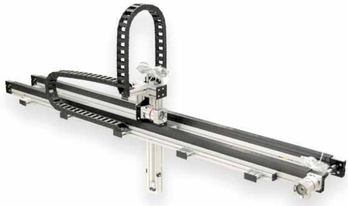
Figure 4: Servo-controlled gantry systems can be used for adhesive dispensing. Photo: Courtesy Macron Dynamics
