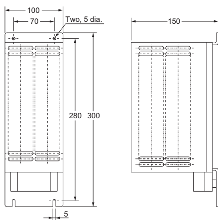
3G3AX-RBC4001
