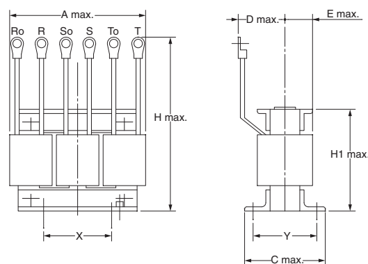
3G3AX-AL4220/3G3AX-AL4330
