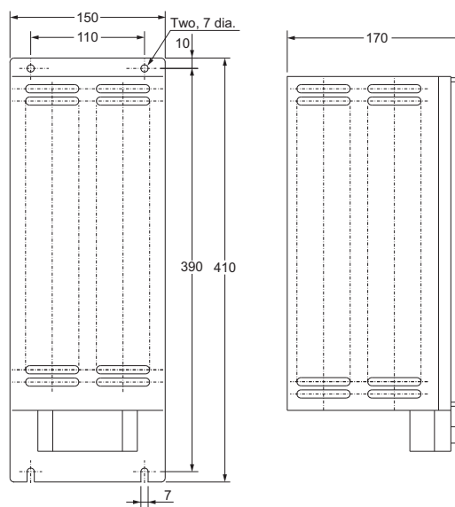
3G3AX-RBC12001
