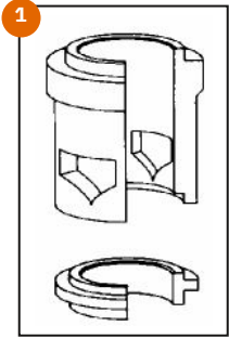
Figure 1. Metal Seat Ring and Ported Cage
