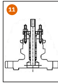
Figure 11. Plain Bonnet
