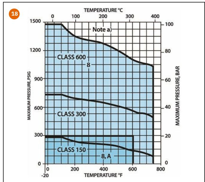
Figure 19. Trim Chart for Chrome Moly Body (ASTM A217, WC9)
