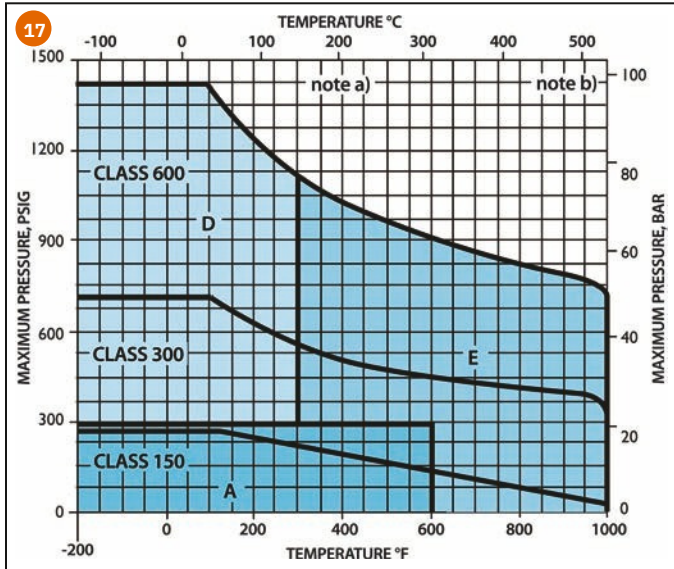
Figure 17. Trim Chart for Stainless Steel Body (ASTM A351, CF8M)
