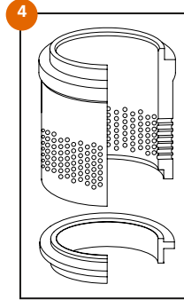
Figure 4. Q-Cage™
