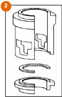
Figure 2. Soft-Seat Ring and Ported Cage
