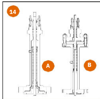
Figure 14. Bellows Seal Bonnets
