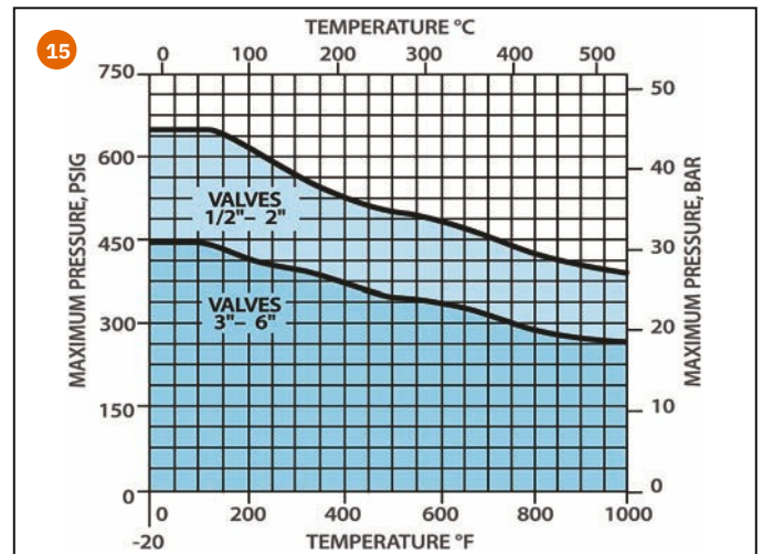
Figure 15. Bellows Seal Rating Chart
