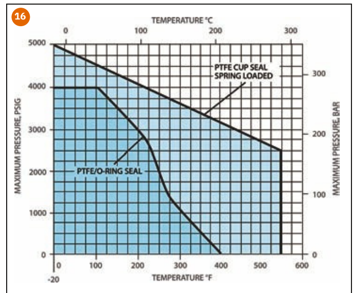
Figure 16. TFE Plug Seal Rating Chart
