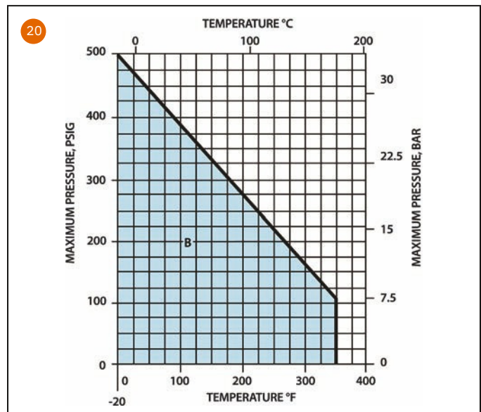
Figure 20. PTFE Soft Seat Rating Chart
