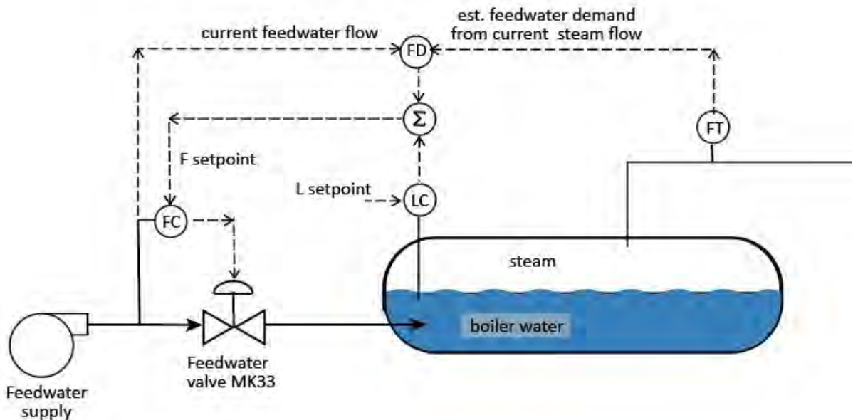
Schematic of a three-element boiler feedwater control loop using a Jordan Mark 33 Valve
