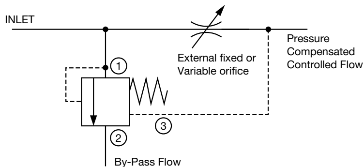
Pressure Compensated Priority Flow Regulator
