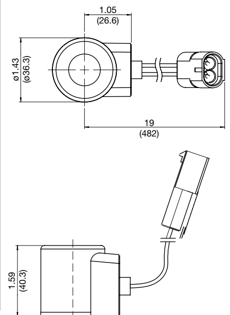
WeatherPak™ 12010973
