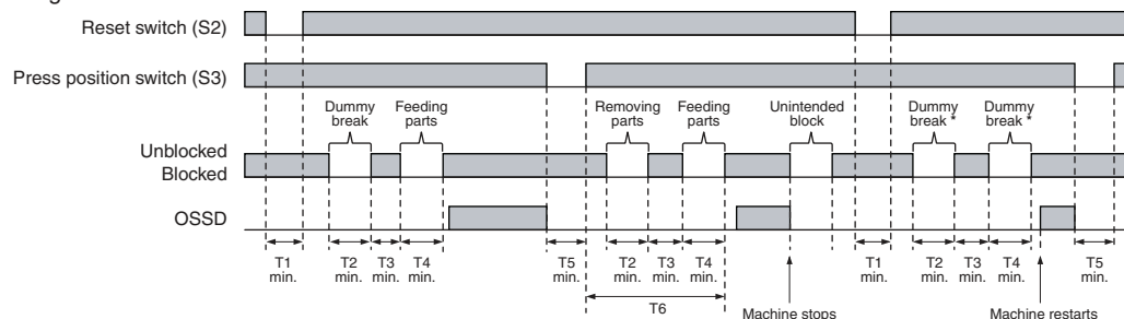
Timing chart
