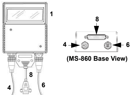
MS-860 Standalone
