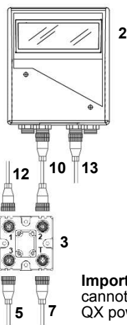
QX-870 Standalone (Serial or Ethernet) with QX-1
